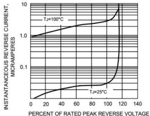
FIG.4-TYPICAL REVERSE CHARACTERISTICS
