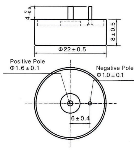
Φ22x8 Layout (B Type)
