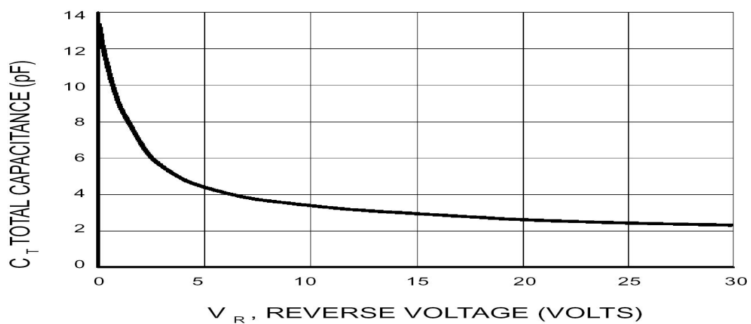
Fig.3 C_T — V_R
